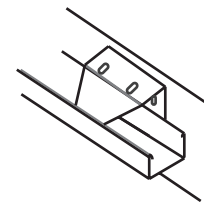
1.3 Centre support bracket installation
