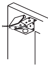
1.2 Bracket installation for outside mount
